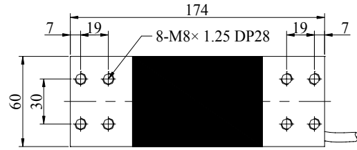
俯视 (Top View)
